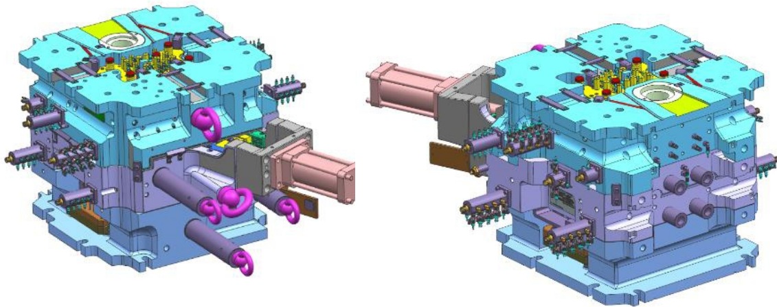
High Pressure Die Casting Die for Crank case
