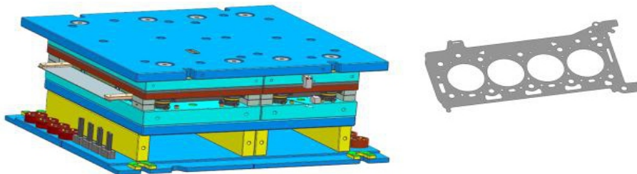
RH Progressive Tool for Gasket
